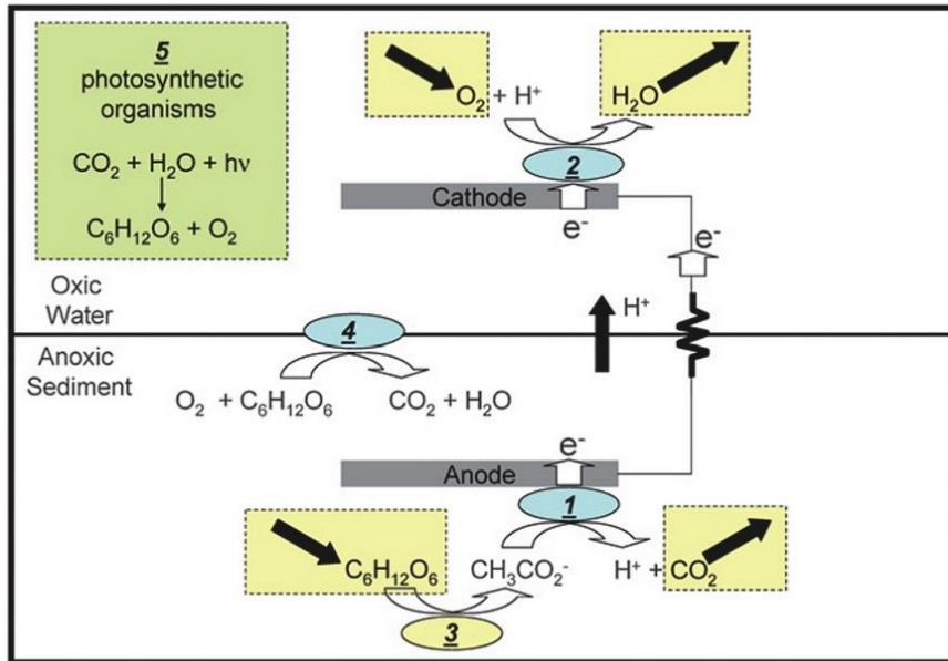
Figure 4 – Solar Microbial Fuel Cell - 2017
